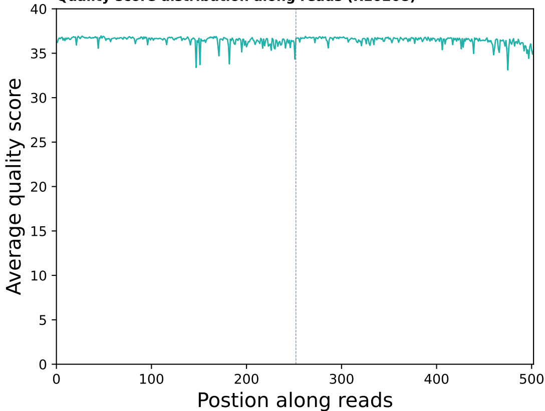
Quality score distribution along reads (R10208)
